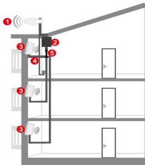
Multi-storey building
