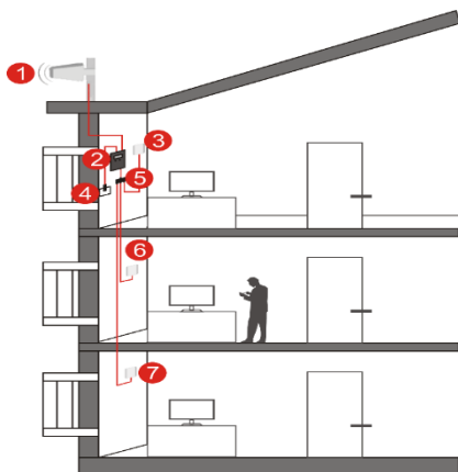
1-Outdoor directional antenna 2- Booster 3, 6, 7- Indoor panel/omni antennas 4-Power supply 5-3-way splitter
