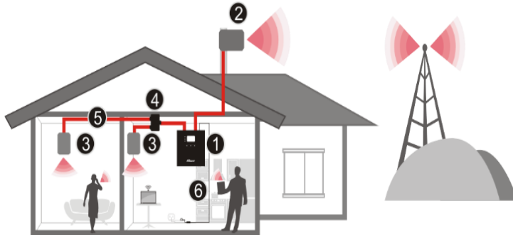
1-Booster 2-Outdoor directional antenna 3- Indoor panel/omni antenna 4-2-way splitter 5-cable 6-power supply
